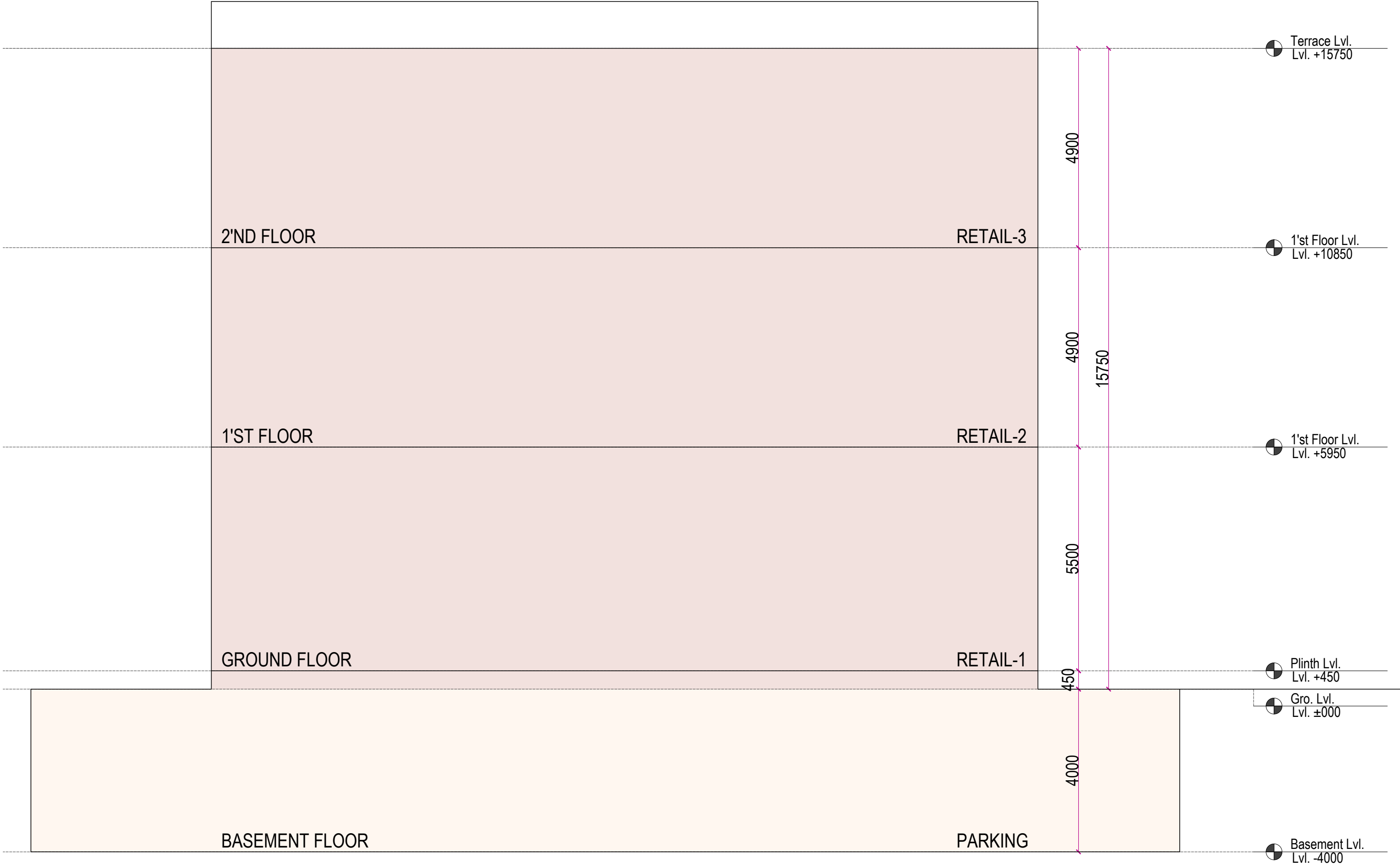
FRONT COMMERCIAL SECTION
