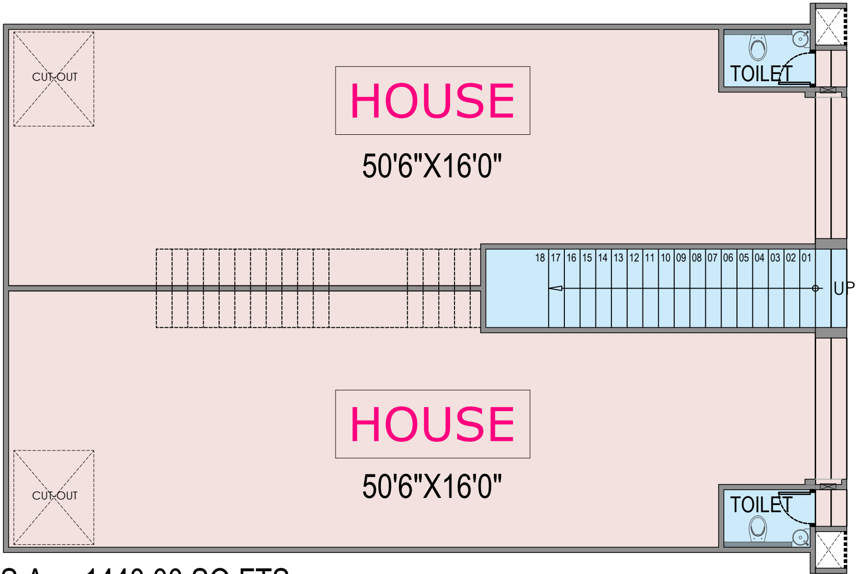
S.A. = 1440.00 SQ.FTS. GROUND FLOOR PLAN
