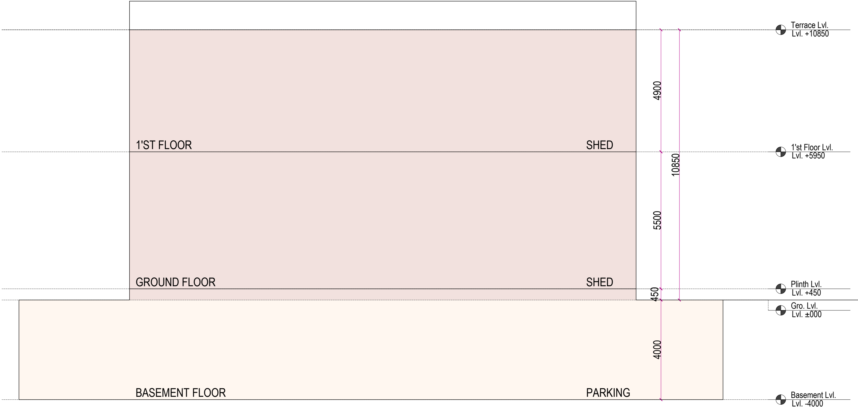
IND. SHED SECTION
